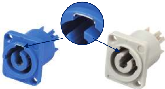
K7122JB/3P-BL
