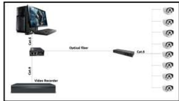
ITEM:K8360TE18A 8P Network optoelectronic converter, optical fiber transceiver
