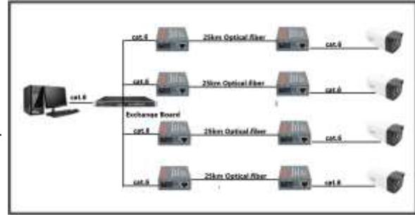
ITEM:K8360TE11A 1P Network optoelectronic converter, optical fiber transceiver
